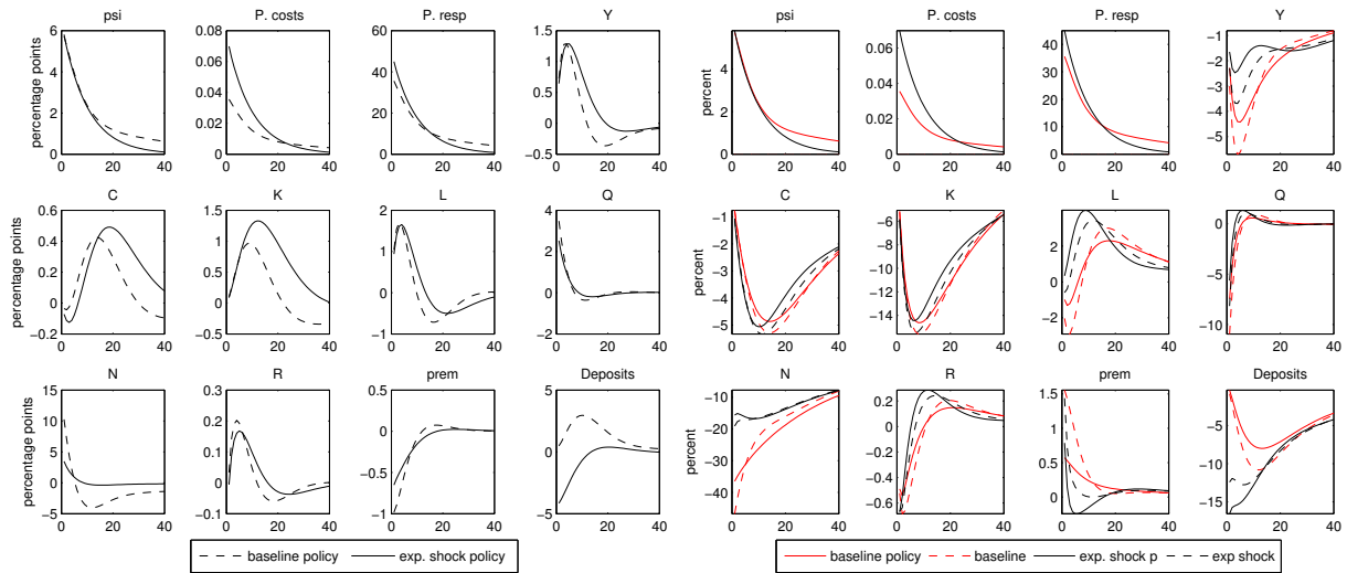
Figure 7: Policy Effects vs Baseline
